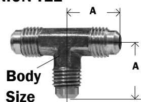
Forged Tee
